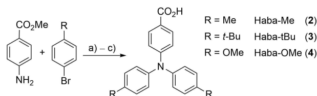
Scheme 2. Preparation scheme for 2–4 : a) \text{Pd}/\text{P}(\text{t-Bu})_3 ; \text{Cs}_2\text{CO}_3 , toluene, 110^\circ\text{C} , 5–7 d; b) KOH, MeOH, reflux; c) HCl.
